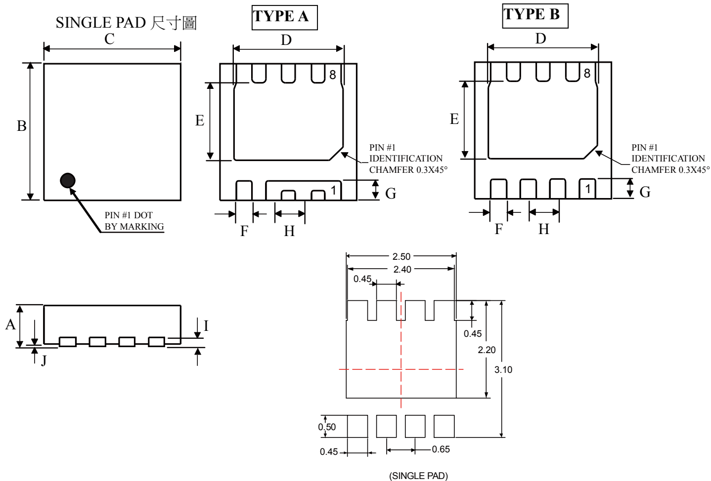
DFN3x3 產品外觀尺寸圖(Product Outline Dimension)
