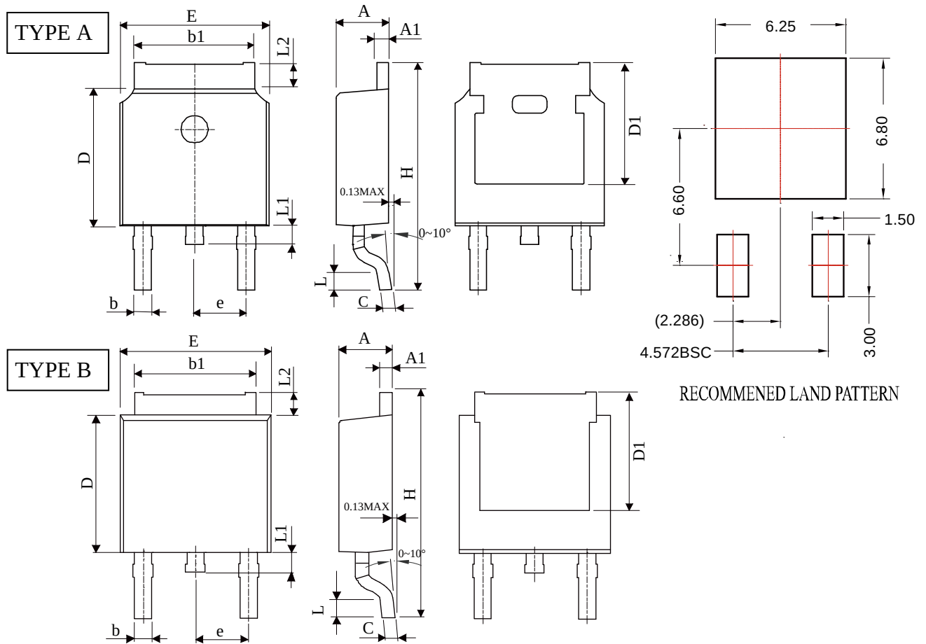
TO-252 產品外觀尺寸圖(Product Outline Dimension)
