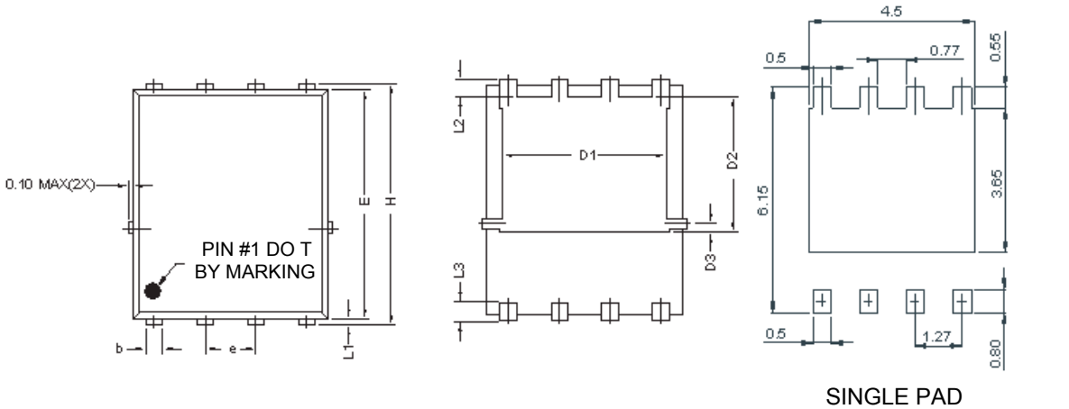
SINGLE PAD RECOMMENDED LAND PATTERN
