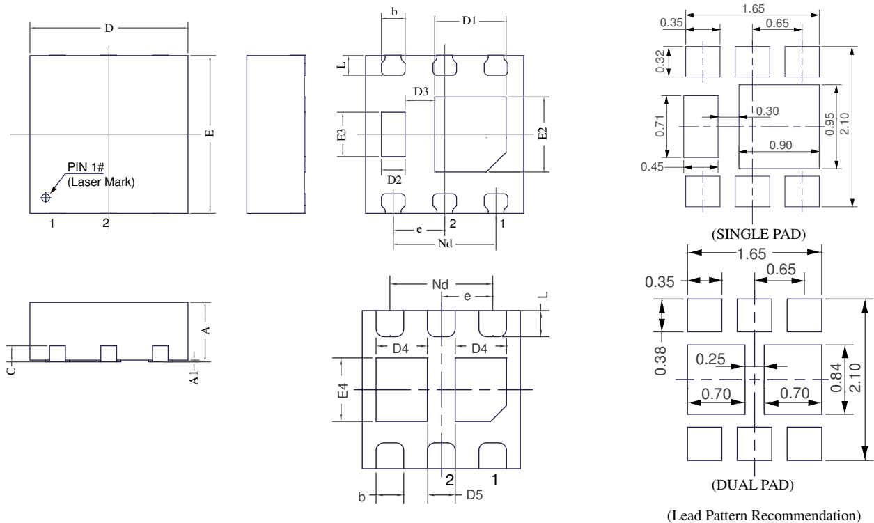
DFN2x2 產品外觀尺寸圖(Product Outline Dimension)
