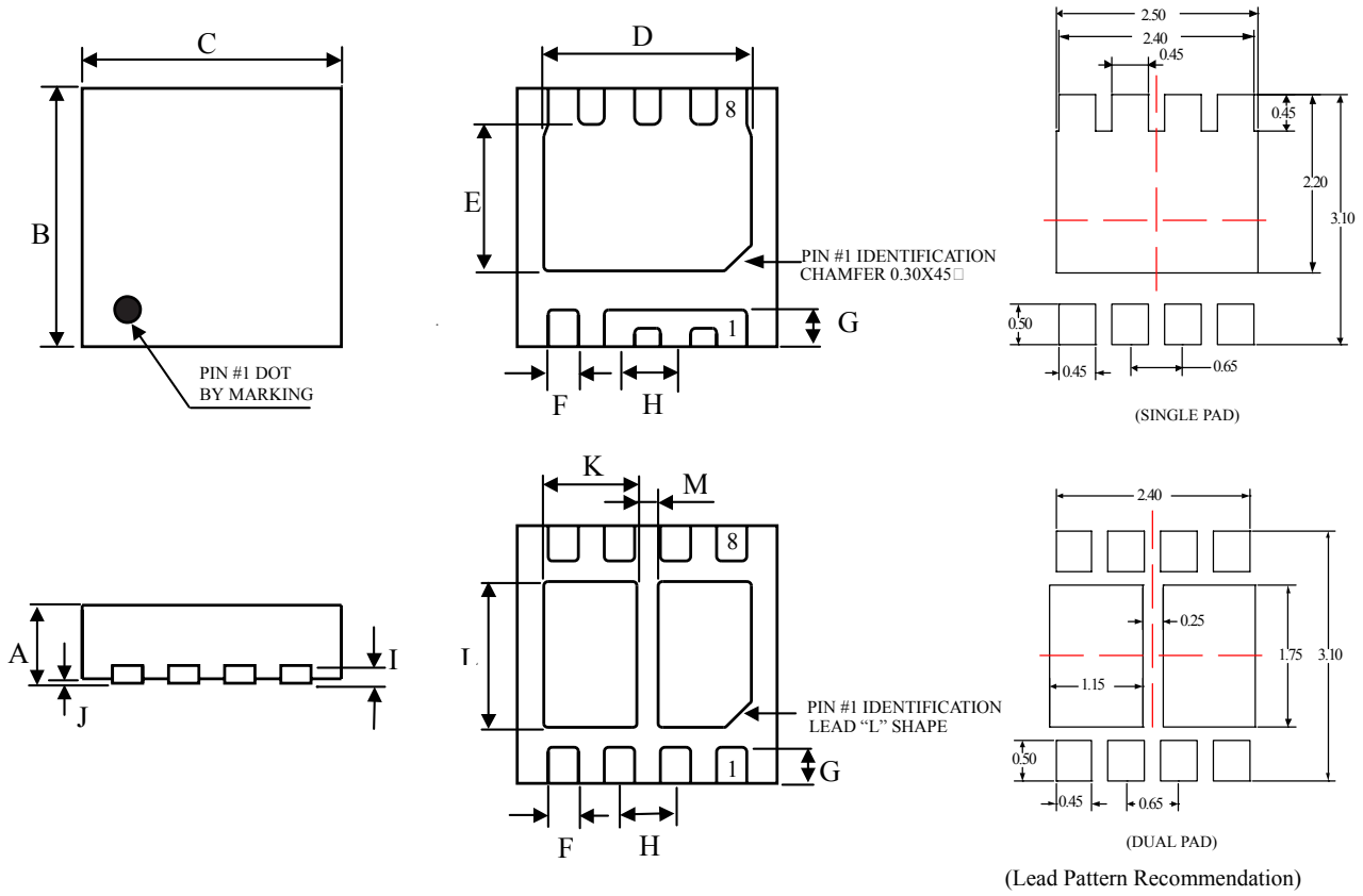
DFN3x3 產品外觀尺寸圖(Product Outline Dimension)
