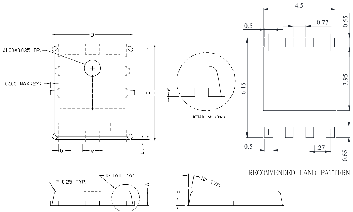
PR-PACK5X6 產品外觀尺寸圖(Product Outline Dimension)
