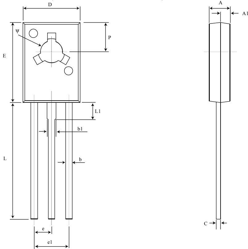
TO-126 產品外觀尺寸圖(Product Outline Dimension)
