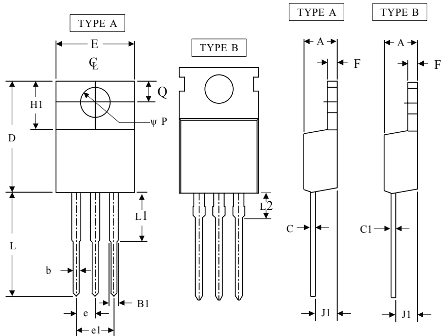
TO-220 產品外觀尺寸圖(Product Outline Dimension)
