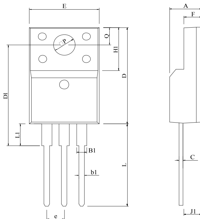
TO-220F 產品外觀尺寸圖(Product Outline Dimension)
