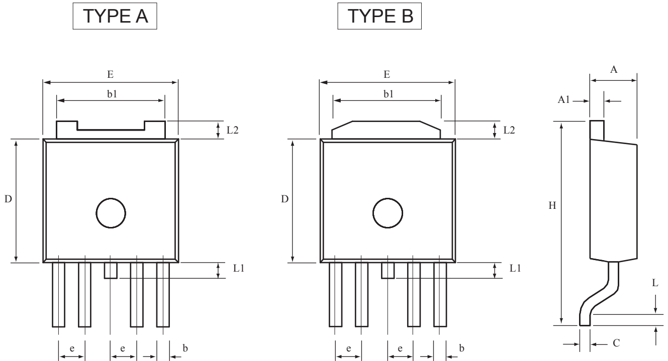
TO-252-4L 產品外觀尺寸圖(Product Outline Dimension)
