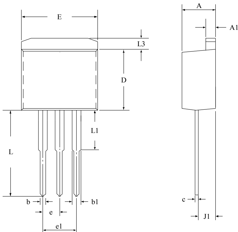
TO-262 產品外觀尺寸圖(Product Outline Dimension)
