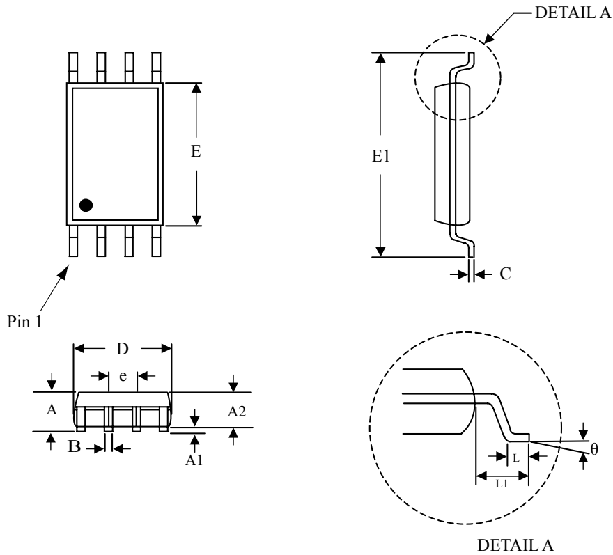
TSSOP-8 產品外觀尺寸圖(Product Outline Dimension)
