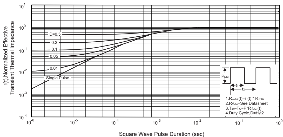
Figure 13. Normalized Thermal Transient Impedance Curve
