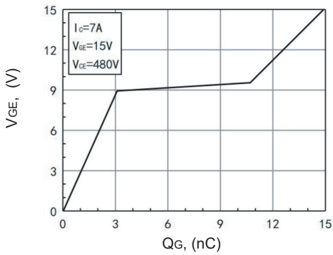
Figure 9. Gate Charge Wave Form
