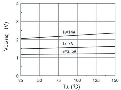
Figure 6. Typical V_{CE(sat)} vs T_J Characteristics
