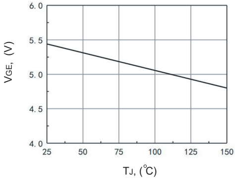
Figure 7. V_{GE(th)} vs T_J Characteristics
