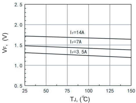
Figure 5. Forward Voltage vs Junction Temperature
