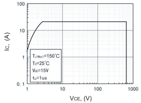
Figure 10. Forward Bias Safe Operating Area
