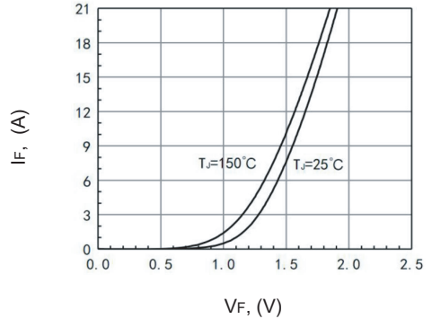
Figure 4. Diode forward current vs forward voltage
