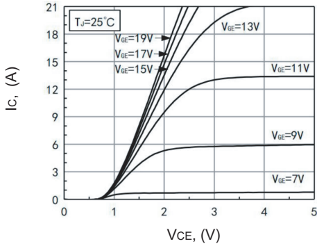
Figure 1. Output Characteristics
