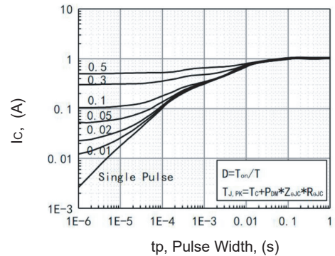
Figure 12. Transient Thermal Resistances
