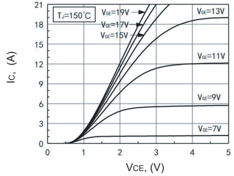
Figure 2. Output Characteristics
