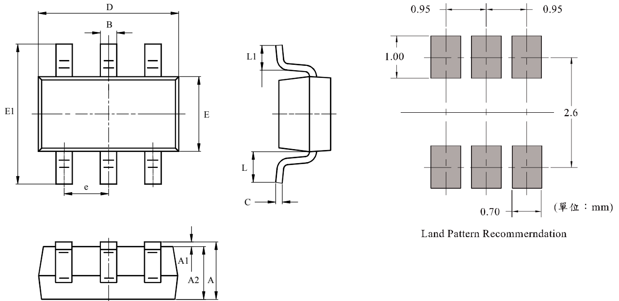
SOT-26 / TSOP-6 產品外觀尺寸圖 (Product Outline Dimension)
