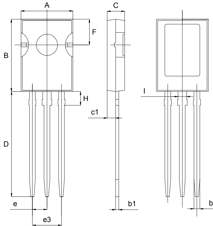
SOT-82 產品外觀尺寸圖(Product Outline Dimension)
