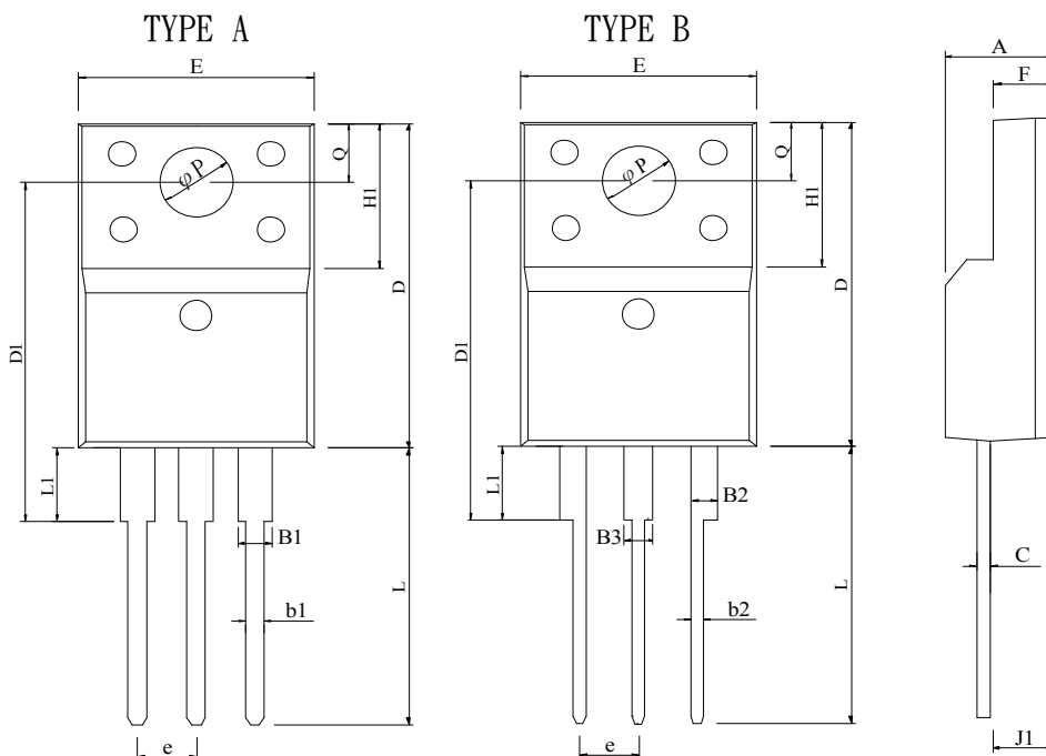
TO-220F 產品外觀尺寸圖(Product Outline Dimension)
