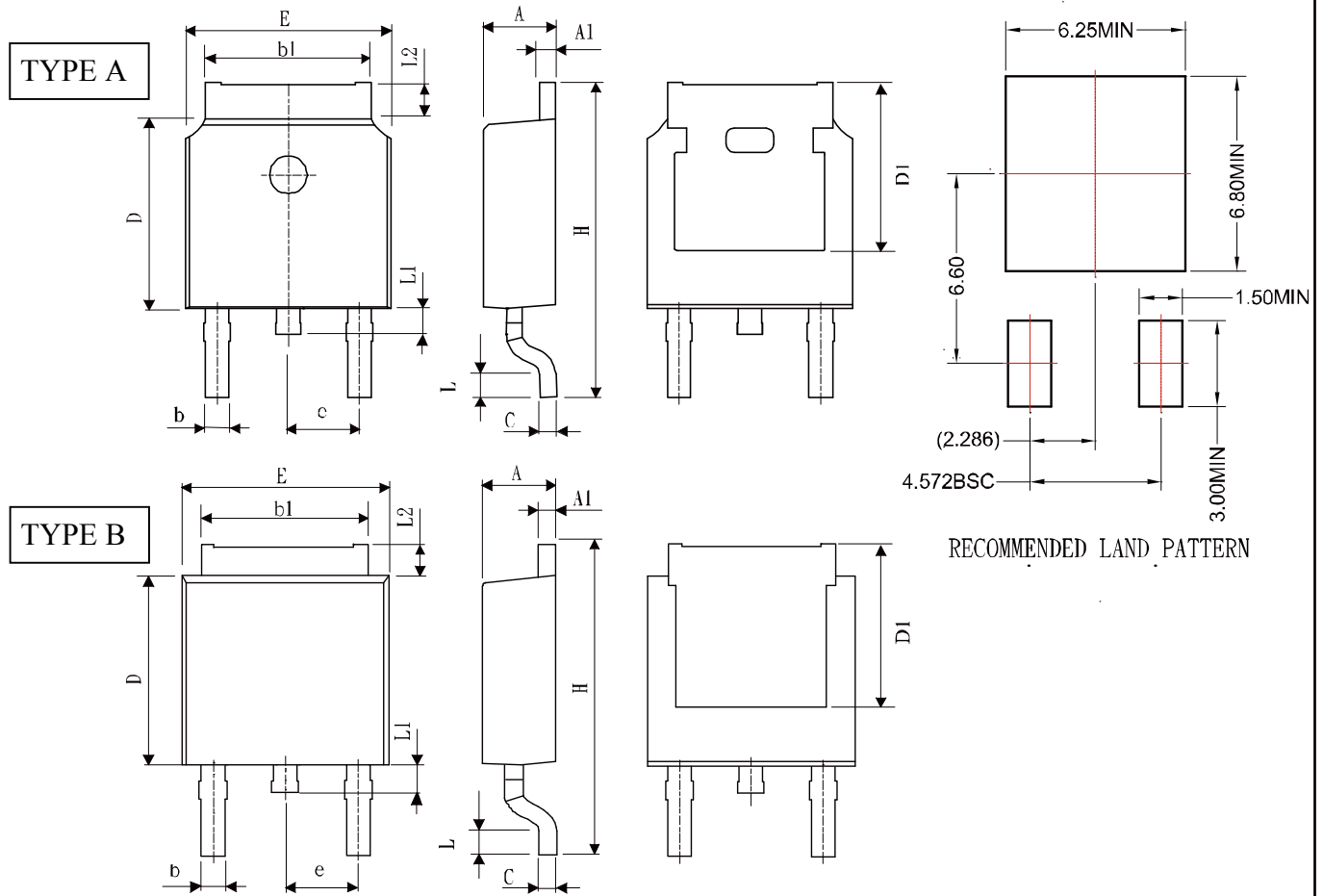
TO-252 產品外觀尺寸圖(Product Outline Dimension)
