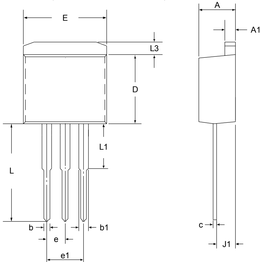
TO-262 產品外觀尺寸圖(Product Outline Dimension)
