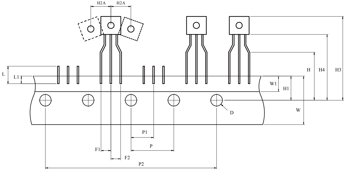
AMMO Packing 包裝示意圖 (AMMO Packing illustration)
