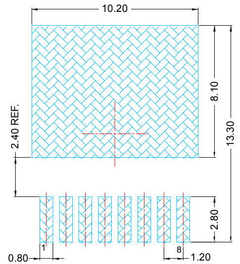
Land Pattern (Only For Reference)
