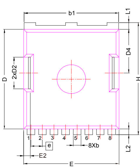
TOLL 產品外觀尺寸圖(Product Outline Dimension)
