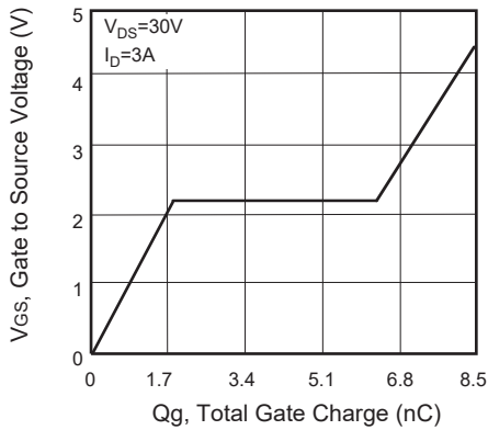
Figure 7. Gate Charge
