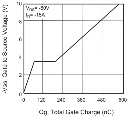
Figure 7. Gate Charge
