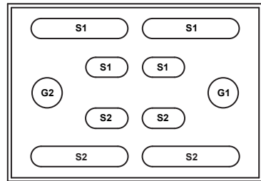
2.08mm*1.45mm WLCSP
